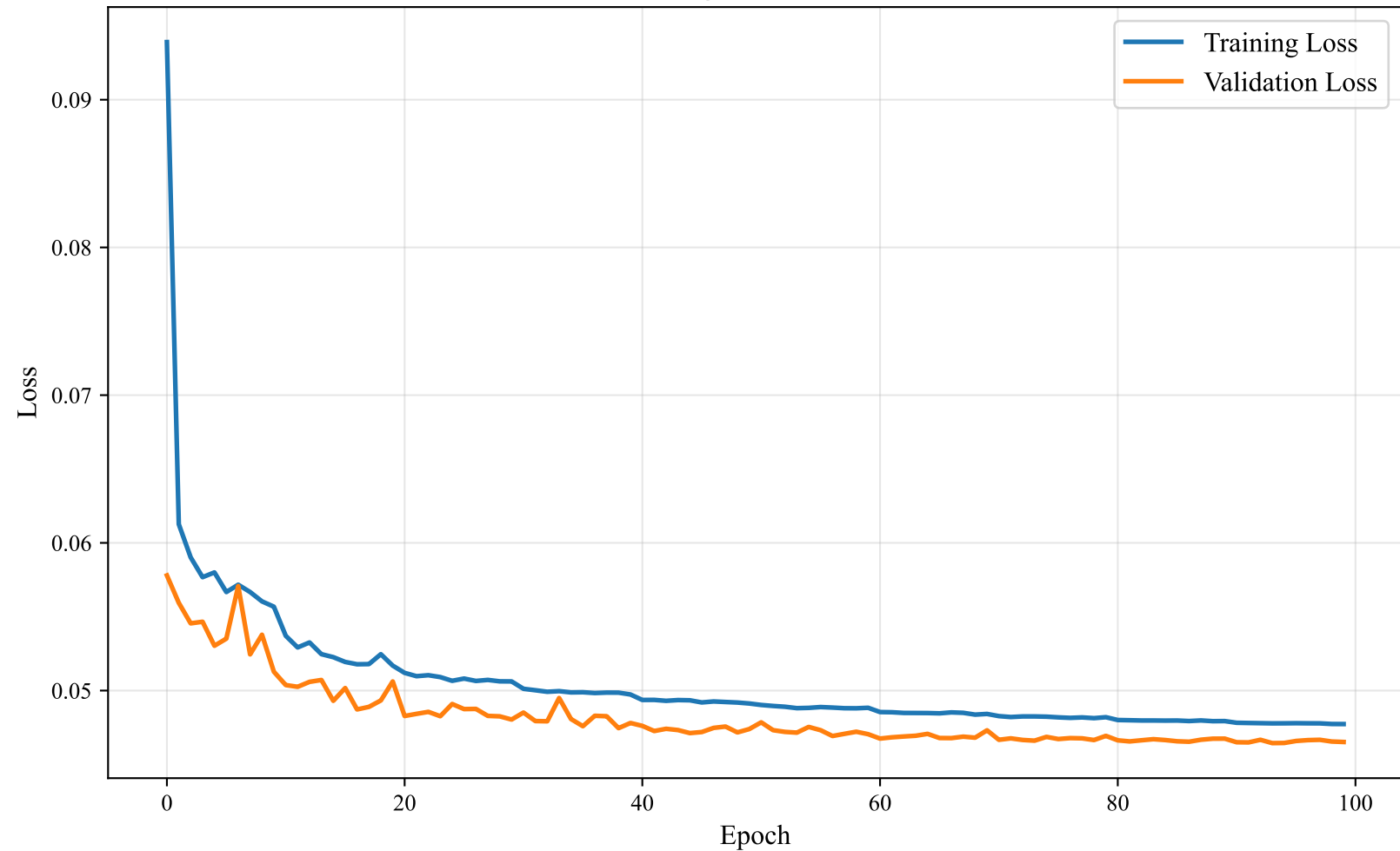
Bi-TSENet Training & Validation Loss - data7
